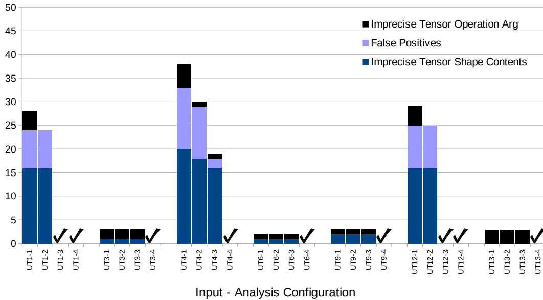
■ Figure 2 Chart: Imprecision metrics under different configurations. Lower is better, check mark is perfect precision. The y axis shows cumulative instances of three imprecision metrics: instances of imprecise tensor arguments, false positives in analysis warnings, and instances of imprecise shapes.
